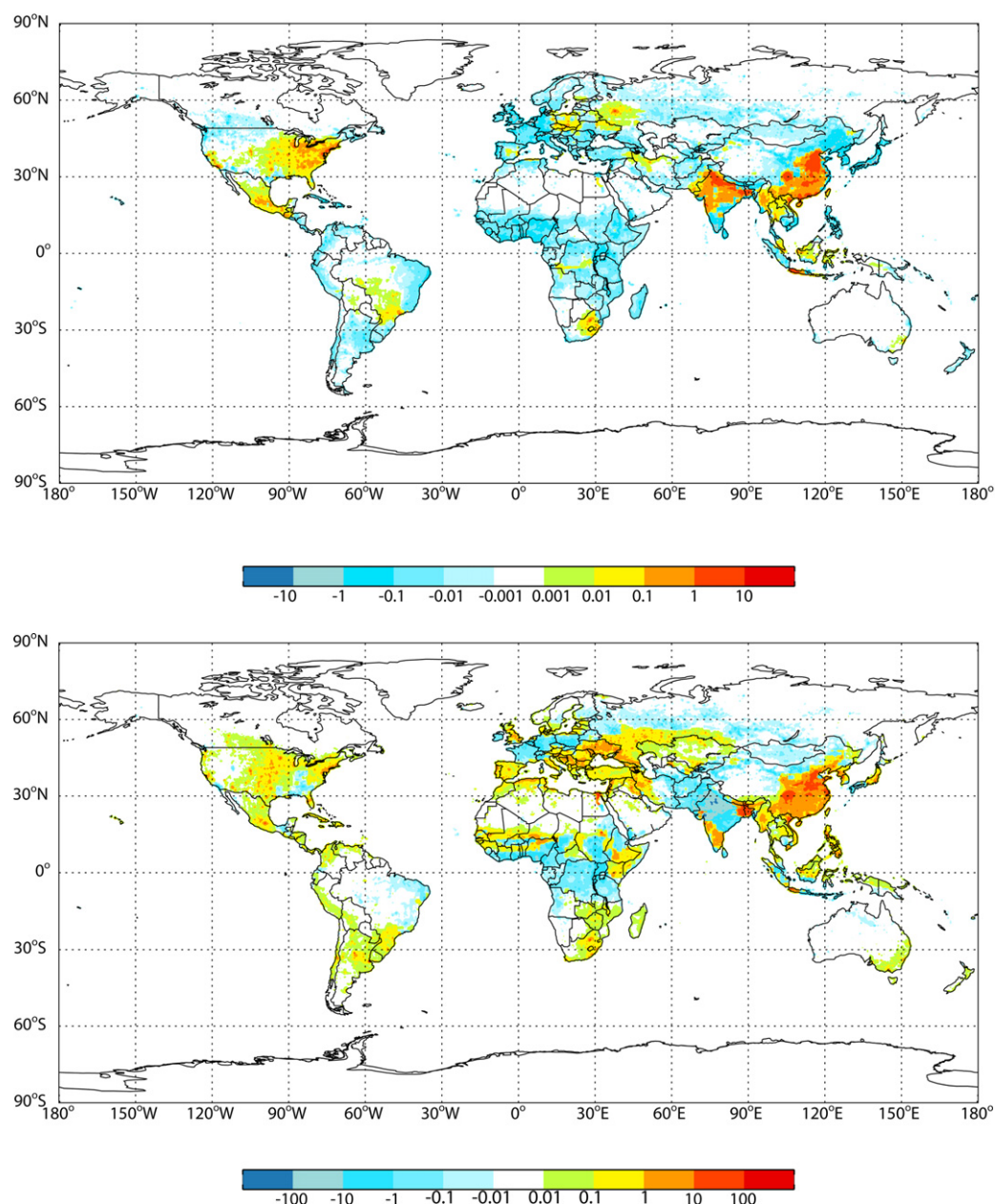
Figure 5. Premature mortality attributable to past climate change (2000–Em2000C11850), in deaths \text{yr}^{-1} ( 1000 \text{ km}^2 ) ^{-1} , for the multi-model mean in each grid cell, for (top) ozone (respiratory mortality) for 9 models and (bottom) \text{PM}_{2.5} (CPD + LC mortality) for the sum of species for 5 models.
