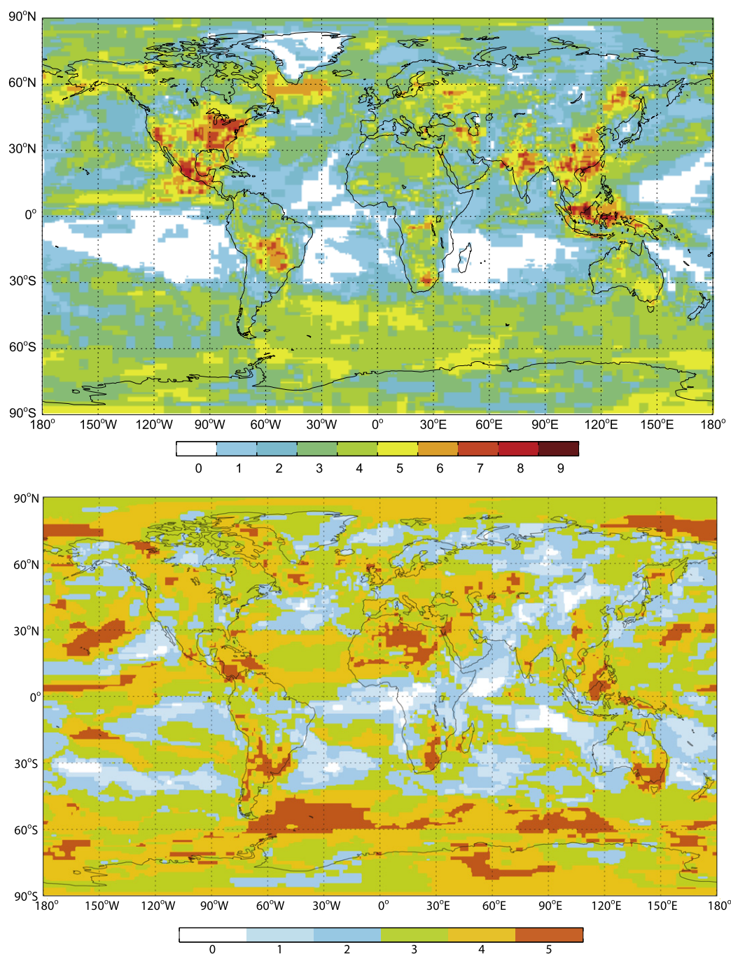
Figure 6. The number of models that show a positive change in concentration in each grid cell due to past climate change (2000–Em2000C1850), for (top) the 6-month ozone season average of 1-h daily maximum ozone (of 9 models total), and (bottom) annual average PM_{2.5} calculated as a sum of species (5 models).
