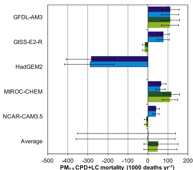
Figure 7. Estimates of the global PM 2.5 CPD and LC mortality attributed to past climate change (2000–Em2000C1850), for PM 2.5 calculated as a sum of species for 5 models (dark blue), and for PM 2.5 as reported by 4 models (dark green). Light-colored bars show the corresponding estimates with a low-concentration threshold (5.8 µg m -3 ). Uncertainty for individual models reflects only the 95% confidence intervals on the CRF (Krewski et al 2009). Uncertainty for the multi-model average is a 95% CI including uncertainty in the CRF and across models.
