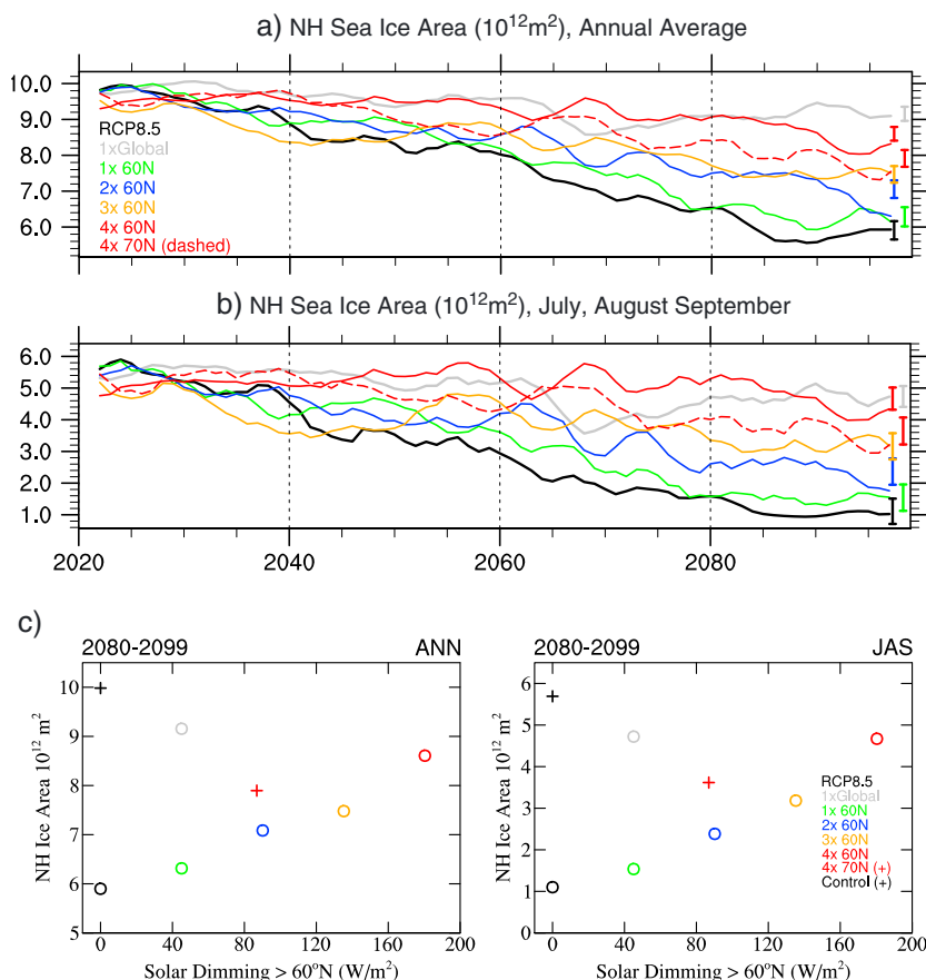
Figure 1. Sea ice area for different model experiments. Evolution of Northern Hemisphere (a) annual average and (b) summer average sea ice area between 2020 and 2100 for different experiments (see legend); a 5 year running mean is applied. The standard deviations of changes with regard to the 5 year running mean are shown on the right of each line, marking the average value derived for the last 20 years of each of the simulations. (c) Scatterplot of NH Ice Area and the downward SW clear sky forcing north of 60°N, for different experiments between 2080 and 2099, (left) annual average and (right) summer average. The forcing of the 4x70N experiment is averaged over 60–90°N.
