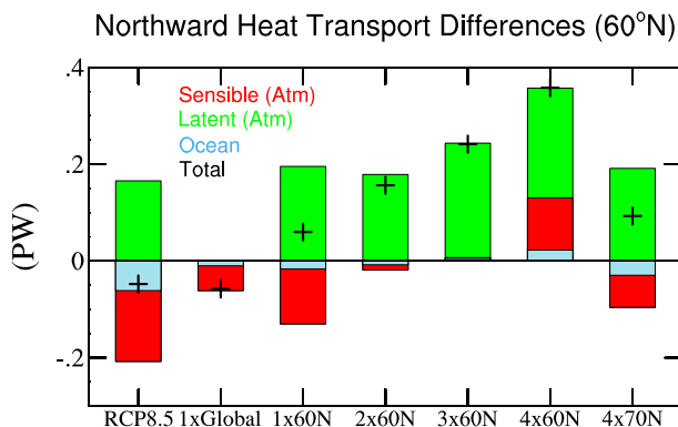
Figure 3. Northward heat transport (NHT) change in Pettawatts at 60°N, relative to the control, for sensible NHT, latent NHT, ocean NHT (colored bars), and total NHT (black plus signs) and for different experiments.
