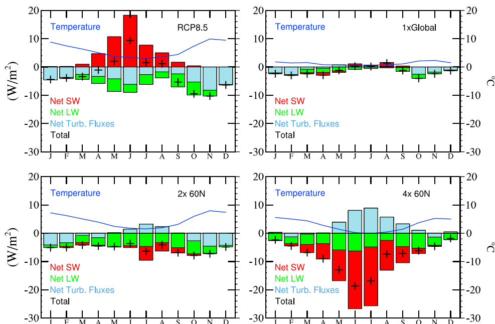
Figure 2. Surface energy budget for different experiments. Seasonal cycle of the Arctic surface heat budget change relative to the control for net shortwave (SW), net long wave (LW), net turbulent (colored bars), total fluxes (black plus signs), and temperature changes relative to the control (blue line), averaged between 60 and 90°N for different experiments (different panels). Flux changes are positive downward.
