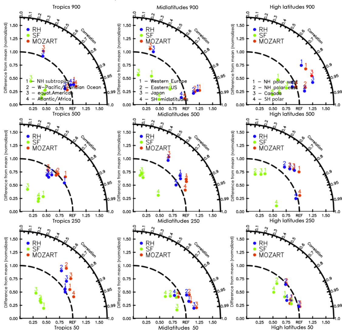
Figure 2. Taylor-like diagrams comparing the mean and correlation of the seasonal cycle between observations (present-day ozone sonde climatology – Tilmes et al., 2012 – from 1995 to 2011 for different regions (tropics, midlatitudes, and high latitudes) and different pressure levels (900, 250, and 50 hPa), as in Fig. 12 of Tilmes et al., 2015, and simulations (red: MO; blue: RH; green: SF).
