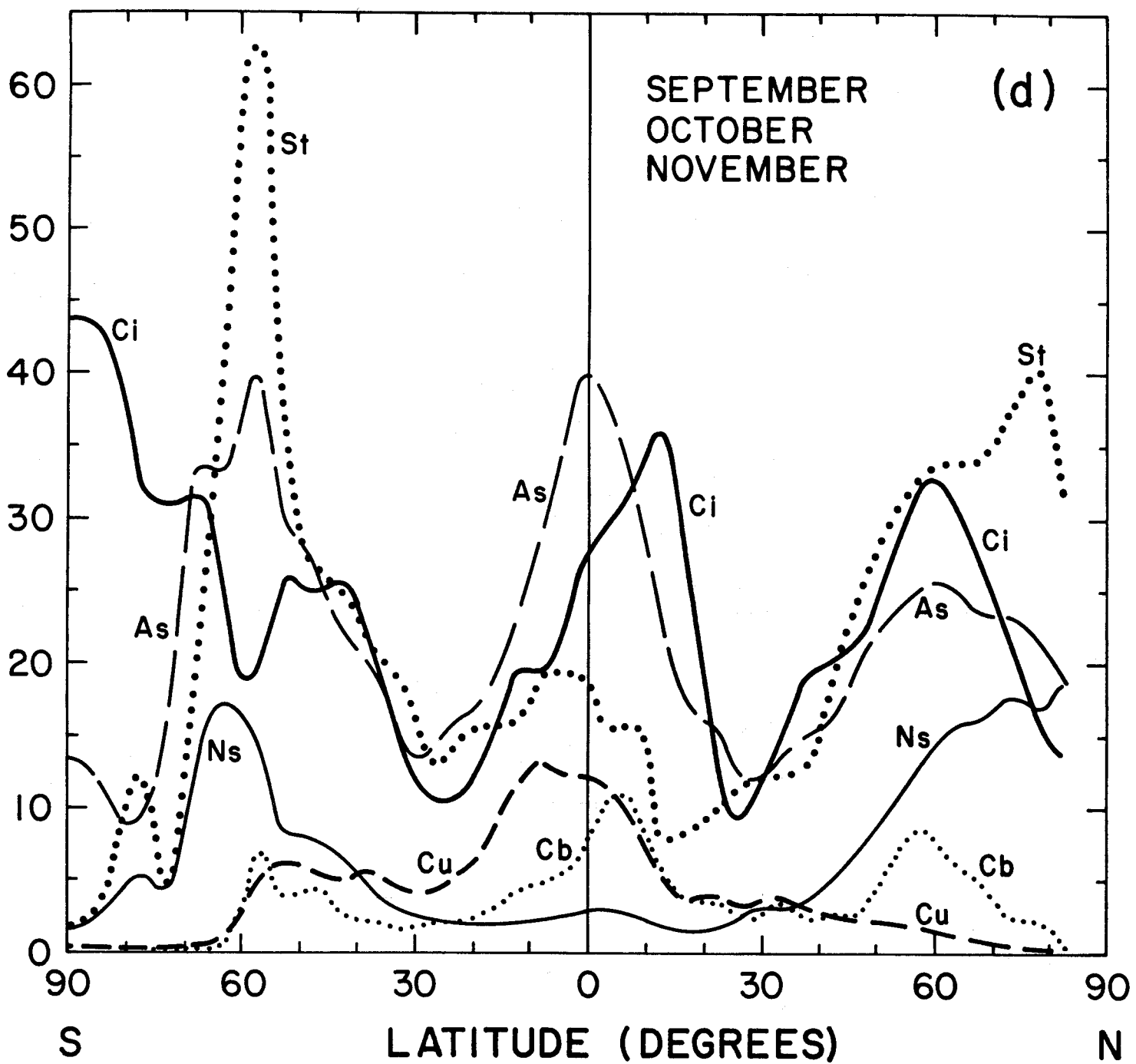
Figure 7. Zonal average amount of each cloud type over land as a function of latitude. Smooth curves were drawn through the data points for 5-degree zones listed on the right side of maps 52-55, 80-83, 108-111, 136-139, 160-163, and 176-179.
