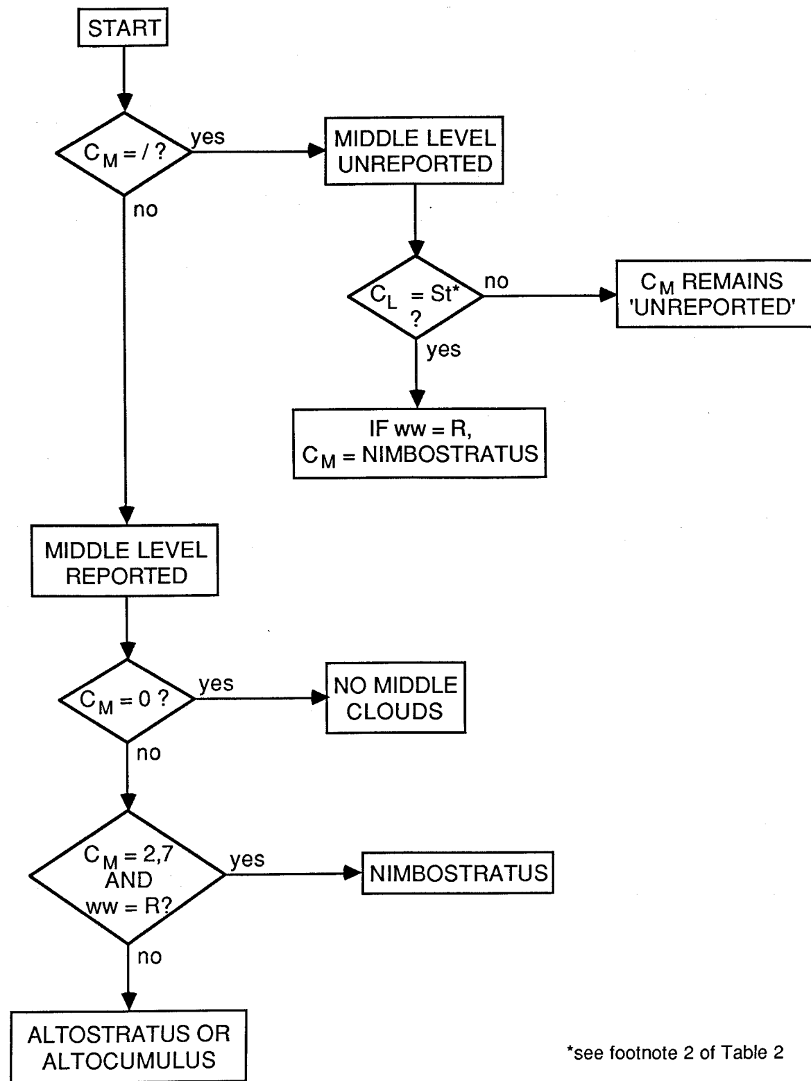
Figure 3. Middle cloud type classification. This figure is the same as Figure 3 of Hahn et al (1984), except for a misprint at the top of that figure which is corrected here.
